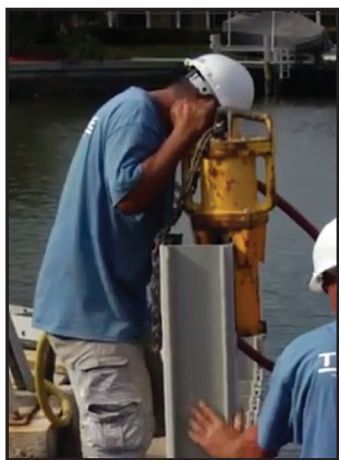
Slotted Master Chuck (P/N 070597) Attached for driving sheet pile.
